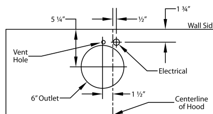
300 CFM B100 Single Blower (Top View)
